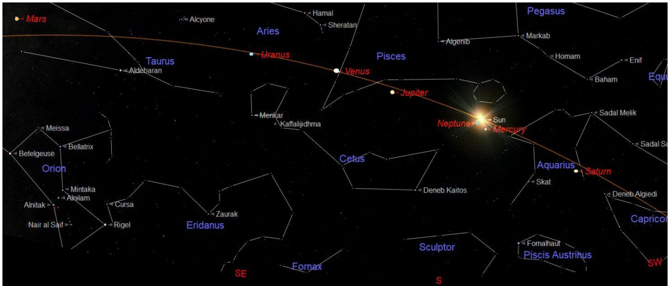
The planets at midday on 15 th March
