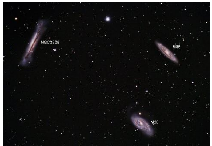
Galaxies M65, M66 and NGC3628 in Leo
