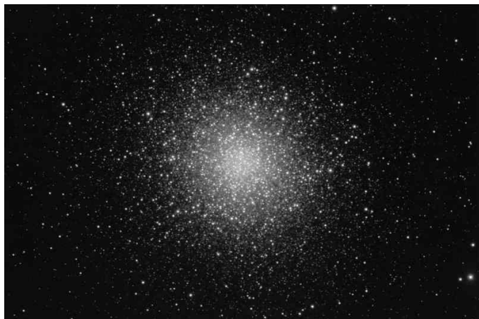
The Great Globular Cluster M13 in Hercules
